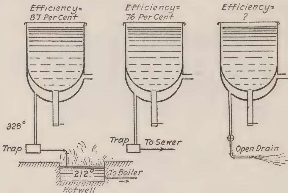
FIG. 6. DRAINAGE SYSTEMS FOR JACKETED KETTLES
